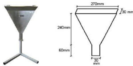
Figure2: V-funnel
