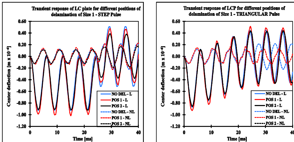
Figure 3. Influence of delamination position on linear and nonlinear transient response
