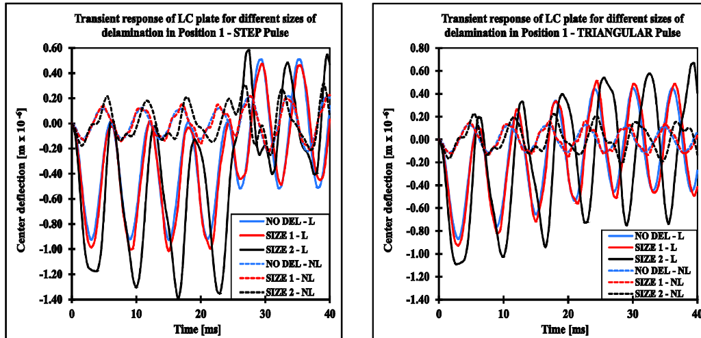
Figure 2. Influence of delamination size on linear and nonlinear transient response
